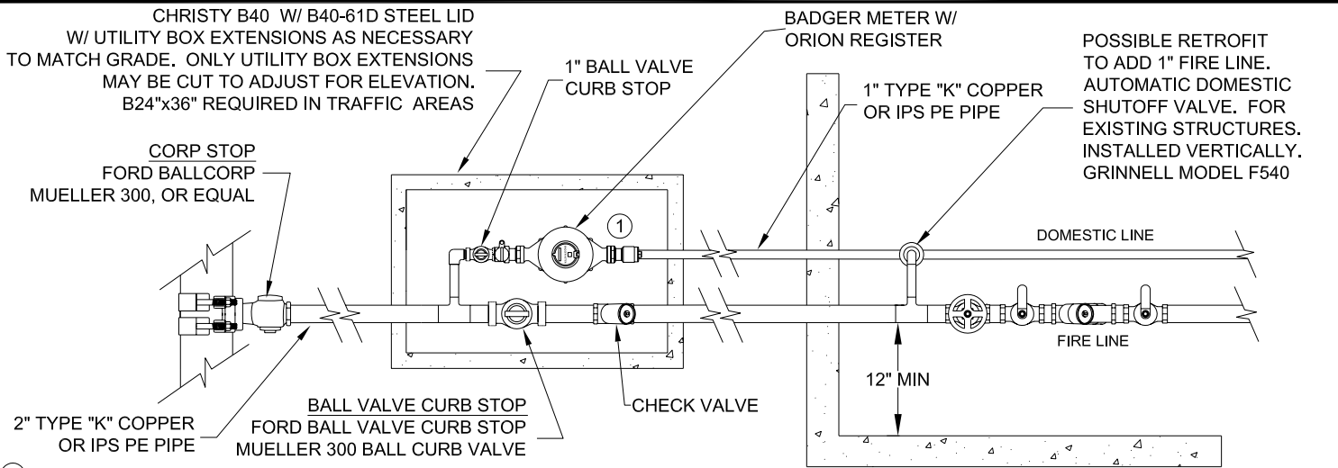
PLAN VIEW
